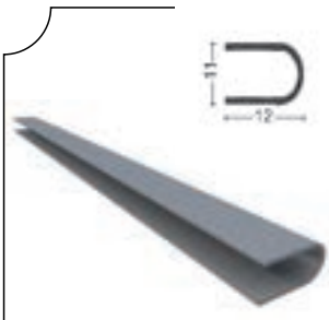
ALMFTL-1005 D Fıtıl Aluminum "D" Seal
