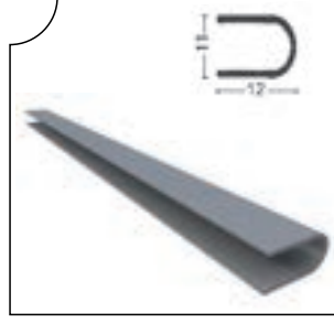
ALMFTL-1005 D Fıtil D Seal
