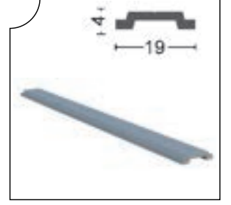
ISICM31-1013 Tij Profili Push Rod Profile
