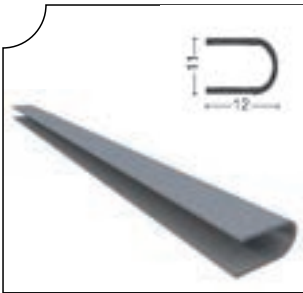
ALMFTL-1005 D Fitiil Aluminum "D" Seal
