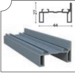
ISICM31-1010 Küçük h Fitil Contalı Esp.Handle Seal (With PVC Seal)
