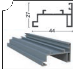
PRGLD-1006 Kollu Fitil Karşılığı Contalı Esp.Handle Opposite Alm. Seal (With PVC Seal)
