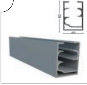
GLDPLS-1001 Kasa Profili Frame Profile
