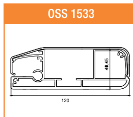
Alt Parça Kapak Bottom Profile Cover
