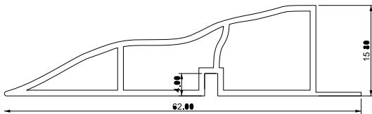
Menfez Kasa Profili Door-way Frame Profile
