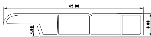
Menfez Kanat Profili Door-way Slat Profile
