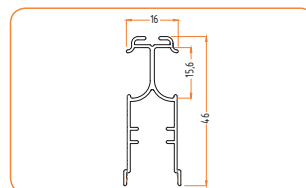
Kanat Profili Wing Profile
