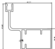
Kulaklı Kapi Kasa Profili Ear Door Frame Profile
