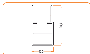
Kasa Profili Frame Profile
